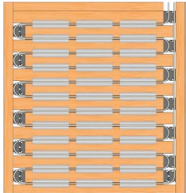
Serpentine Loop - primarily used with solid hardwood flooring
